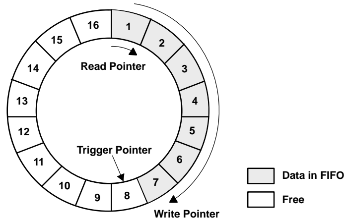
Figure 29. Circular Buffer
