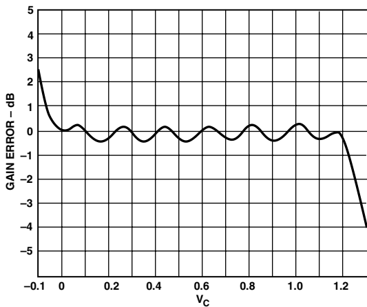
Figure 7. Gain Error for Cascaded Stages—Parallel Control
