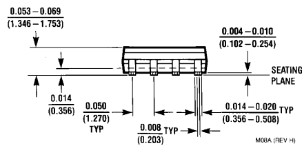
8-Lead (0.150" Wide) Molded Small Outline Package, JEDEC Order Number LM4880M NS Package Number M08A
