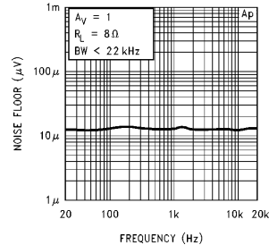
Noise Floor
