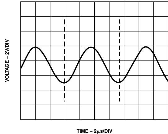
Figure 8. Output of Wien Bridge Oscillator
