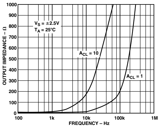
TPC 21. Output Impedance vs. Frequency
