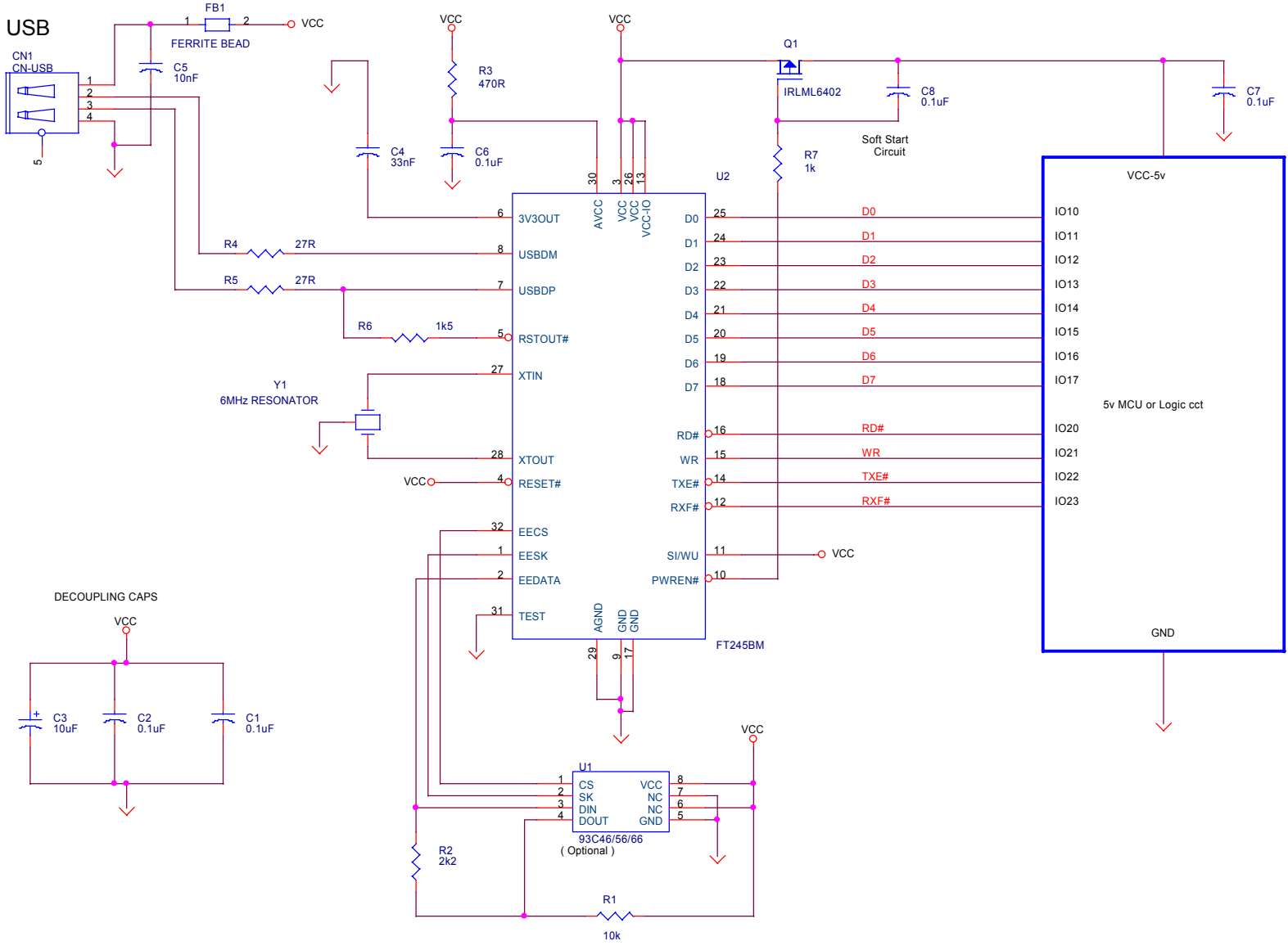
FT245BM 5v BUS POWERED EXAMPLE WITH POWER SWITCHING
