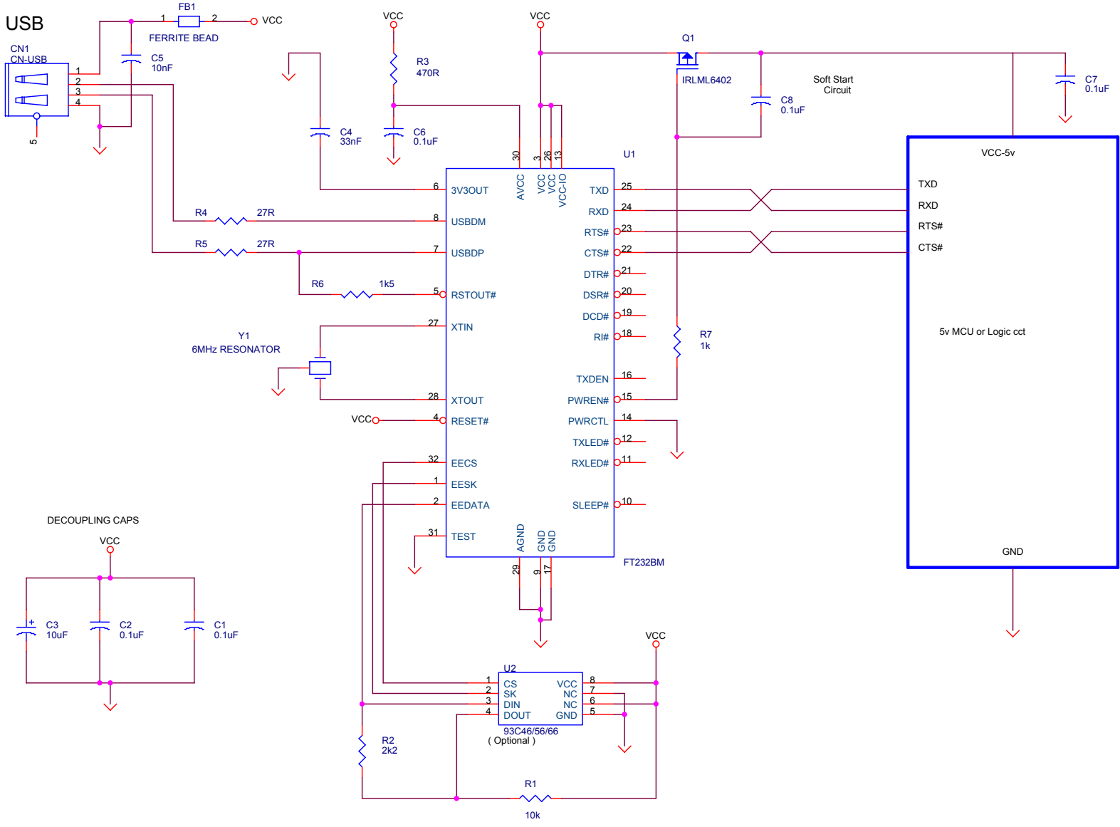
FT232B APPLICATION SCHEMATIC POWERED APPLICATION WITH POWER SWITCHING
