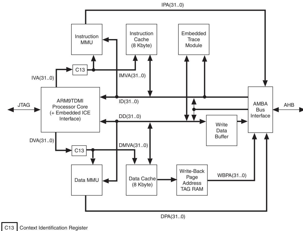
Figure 3. ARM922T-Based Embedded Processor Internal Organization
