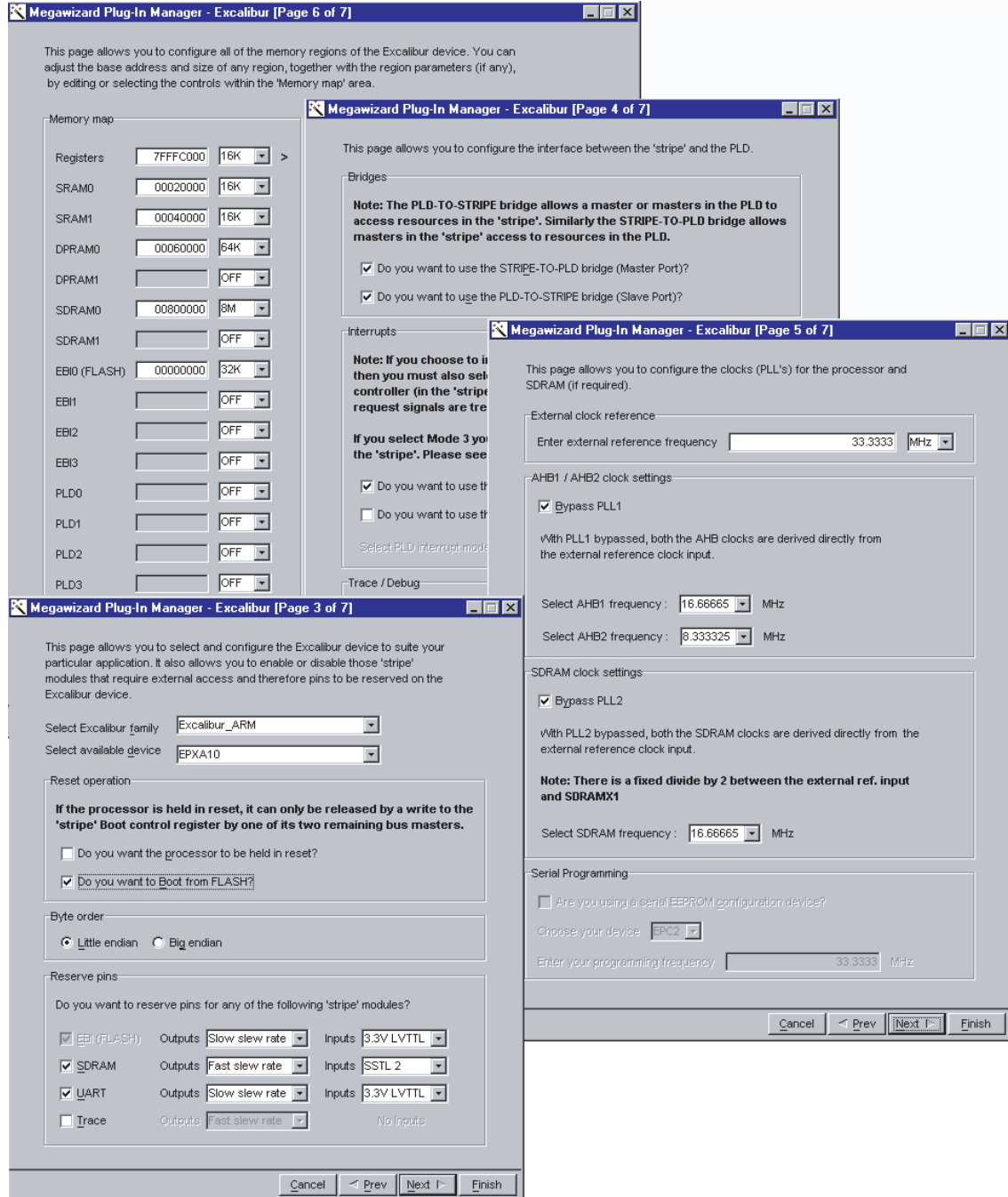
Figure 5. Excalibur Configuration Wizard
