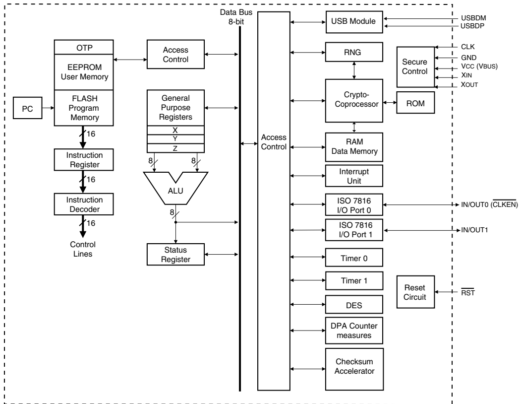
Figure 1. The AT90SC6464C-USB AVR Enhanced RISC Architecture
