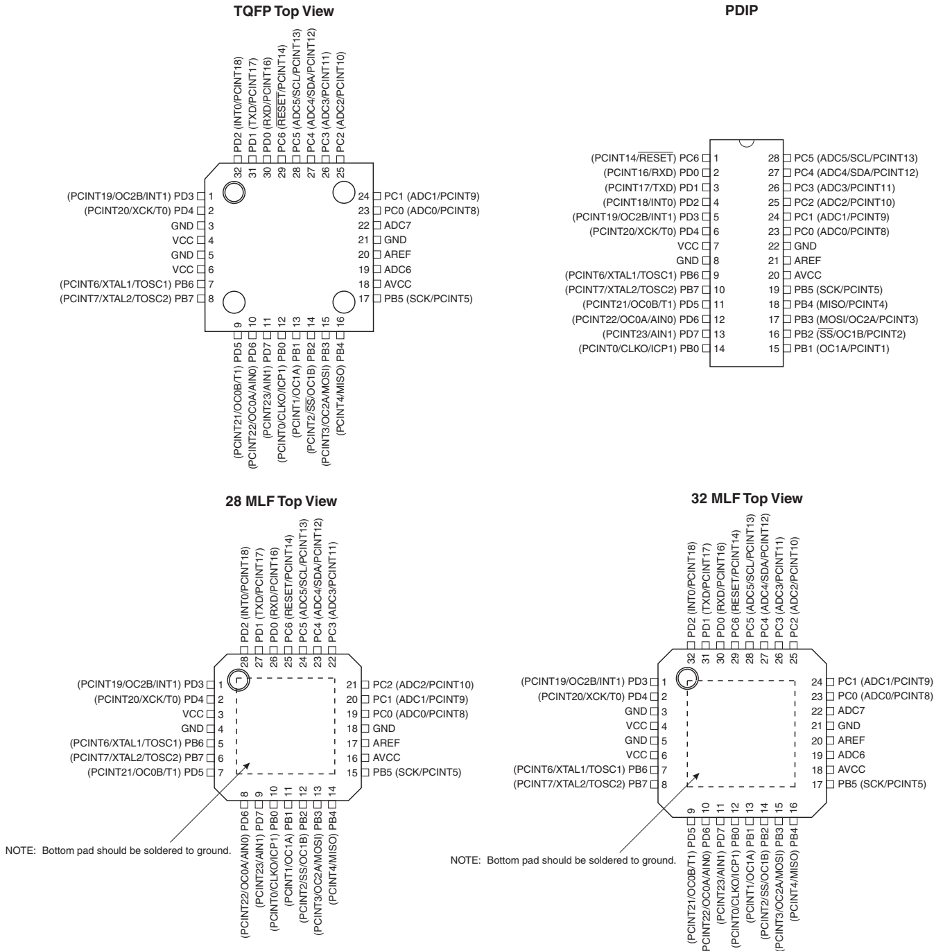
Figure 1-1. Pinout ATmega48/88/1682545RS
